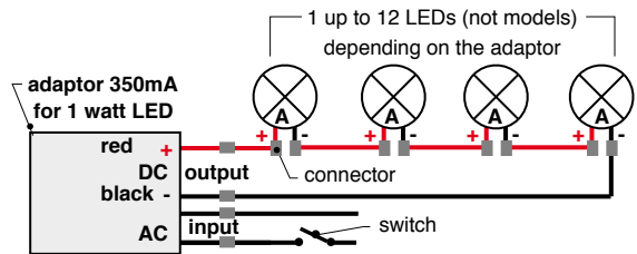
scheme - 1 circuit - not dimmable 1W - 350mA
