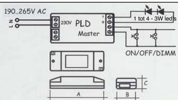
scheme - 1 circuit - dimmable 3W - 700mA
