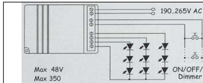
scheme - dimmable ZDBOX30 1W - 350mA
