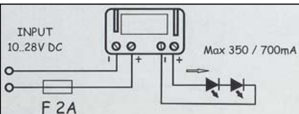
scheme 12 or 24V - not dimmable ZLVQ 12-24V 3W - 700mA
