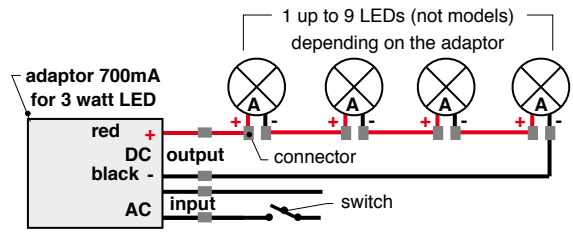
scheme - 1 circuit - not dimmable 3W - 700mA
