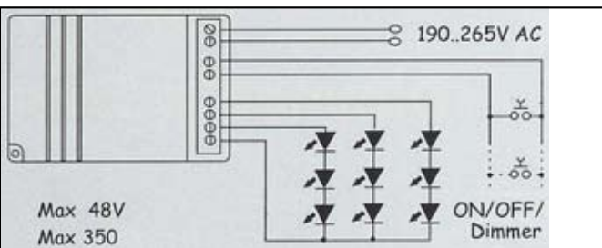
scheme - RGB ZRBOX 1W - 350mA
