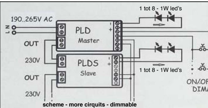
scheme - more circuits - dimmable 1W - 350mA
