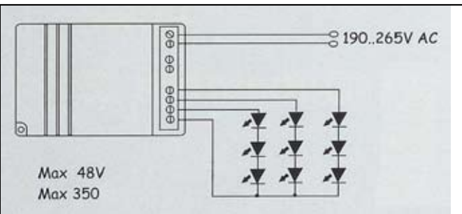
scheme - not dimmable: ZDBOX30 SP 1W - 350mA
