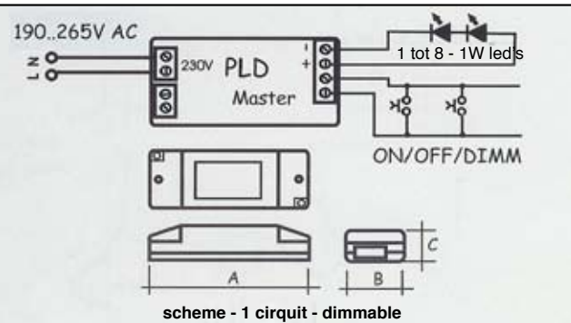
scheme - 1 circuit - dimmable 1W - 350mA
