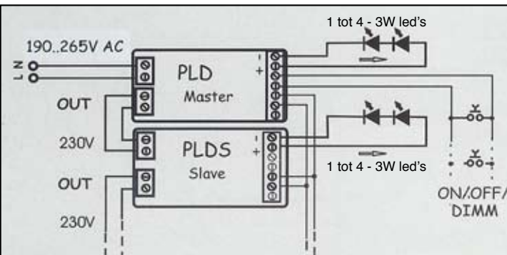
scheme - more circuits - dimmable 3W - 700mA
